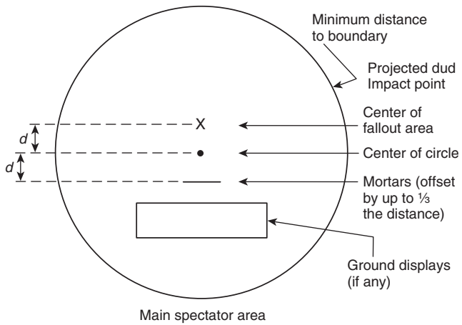
FIGURE A.5.2.1.4.1 Typical Layout for a Display Site Using Angled Mortars. The distance, d , should be at least one-sixth but not more than one-third the radius of the circle, indicating the minimum distance to the secured boundary.
